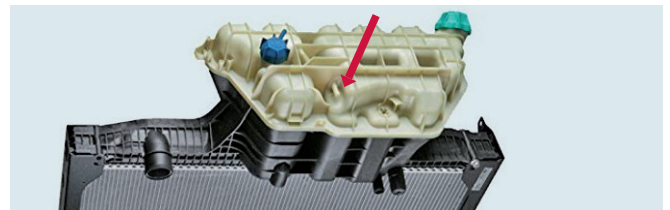
Figure 1: Older-generation expansion tank with one connection
