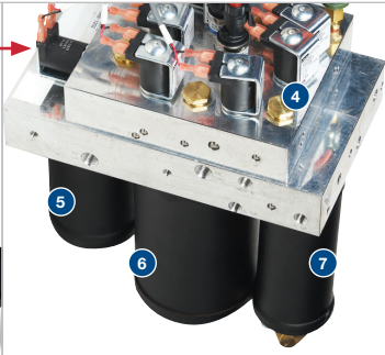
KWIK-CHANGE "Block" Manifold Assembly Patented design for ease of repair, plug and play
