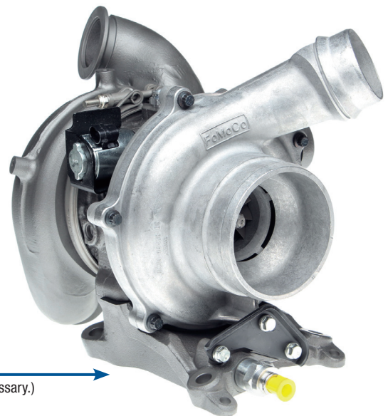
Single Scroll
